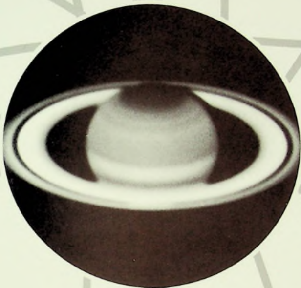
The planet Saturn and its famous ring system as seen through the 100-inch Mt. Wilson telescope. —Mt. Wilson and Palomar Observatories
