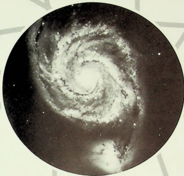
A spiral nebula with satellite nebula in Canes Venatici taken with the 200-inch Hale telescope. —Mt. Wilson and Palomar Observatories
