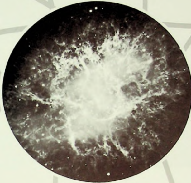
Remains of a supernova which occurred in AD 1054, the "Crab" Nebula in the constellation Taurus . —Mount Wilson and Palomar Observatories
